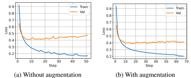
Figure 2. Loss curve of the model trained with and without augmentation
