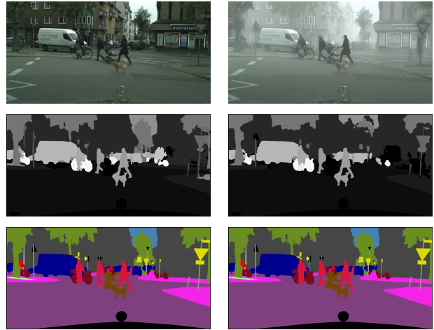
Figure 1. (top) An image from Cityscapes dataset and its foggy version (middle) Semantic segmentation identified for the two images by our model (trained with augmentation) (bottom) ground truth for semantic segmentation of both images
